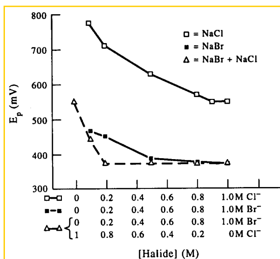
Fig. 6. The variation of E_p with anion concentration for 316 wire in solutions of (□) NaCl, (■) NaBr and (△) mixtures of NaCl and NaBr, pH 5.5.
