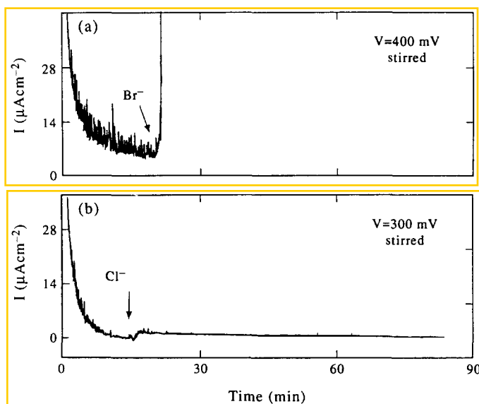
Fig. 7. (a) Current decay profile recorded at a potential of 400 mV(SCE), initially in a 1.0 M NaCl, pH 2.5 solution. NaBr added after a 20 min passivation period. (b) Current decay profile recorded at a potential of 300 mV(SCE) in a 1.0 M NaBr, pH 2.5 solution; 1.0 M NaCl added after a 20 min passivation period.
